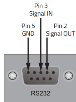
RS232 Terminal Pin-Out
