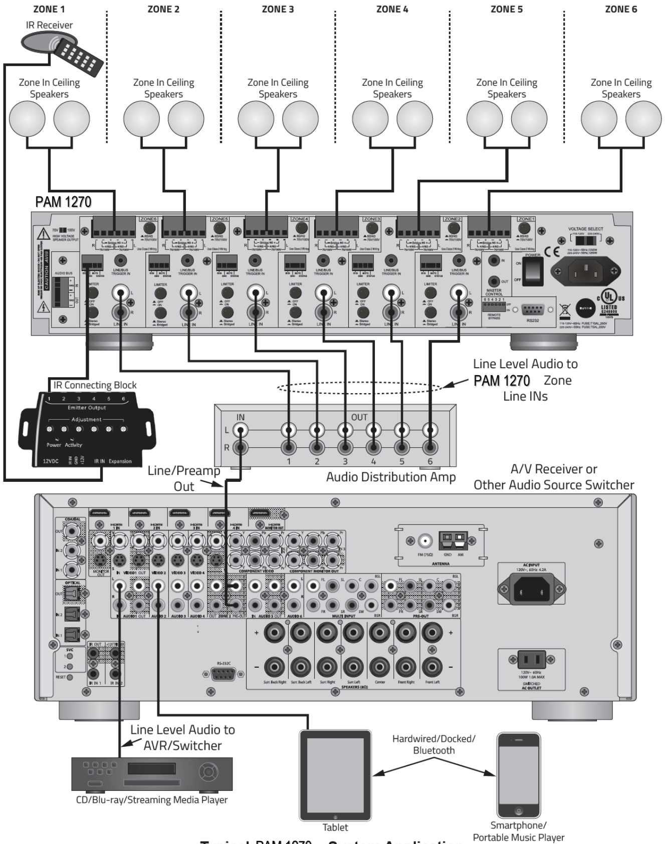
Typical PAM 1270 System Application
