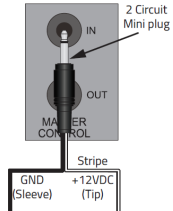
Master Control IN Connection
