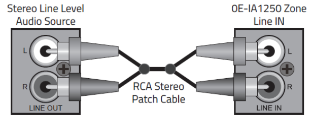
Zone Line IN Connections
