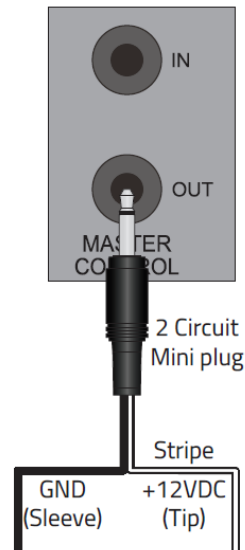
Master Control OUT Connection
