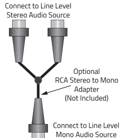
Zone Line IN Connections
