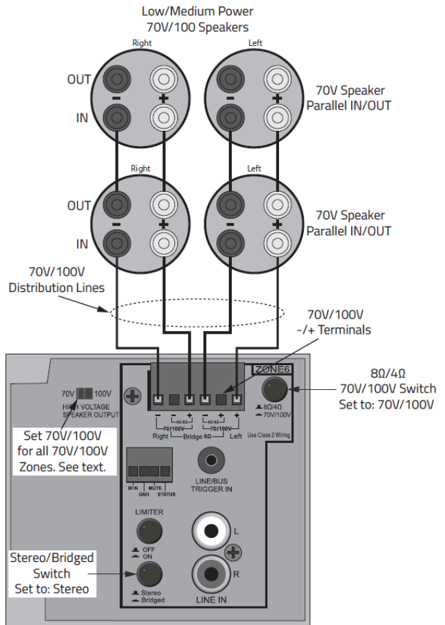
70V/100V Connection
