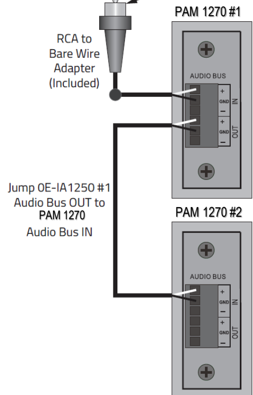
Audio Bus IN/OUT Connections
