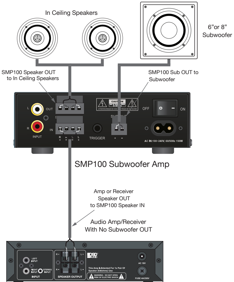
Speaker Level Input Illustration
